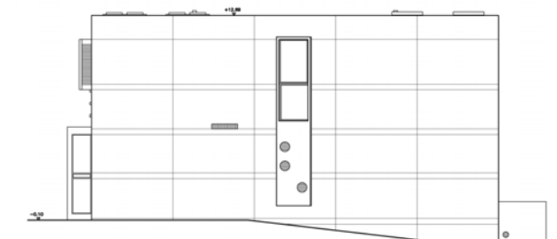
ALZADO SUR/ SOUTH ELEVATION
