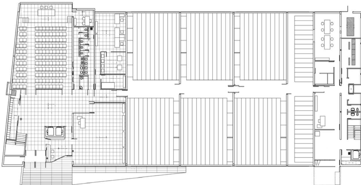
PLANTA BAJA/ GROUND FLOOR PLAN
