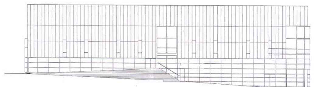
ALZADO NORTE/ NORTH ELEVATION
