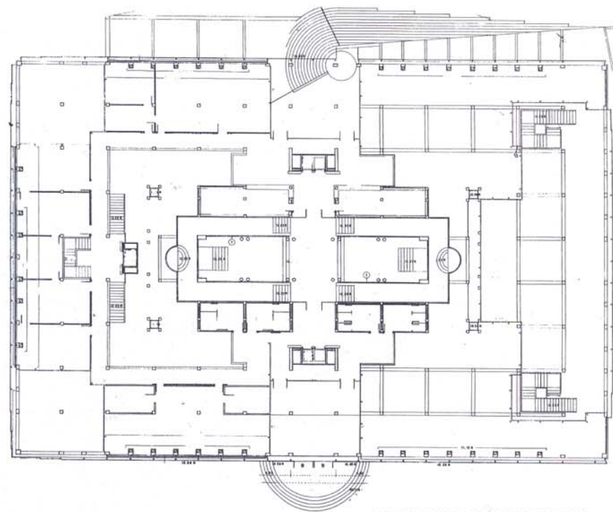
PLANTA PRIMERA/ FIRST FLOOR PLAN
