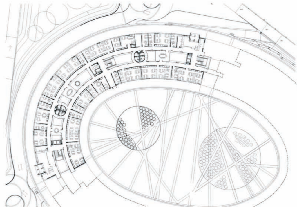
PLANTA BAJA/ GROUND FLOOR PLAN
