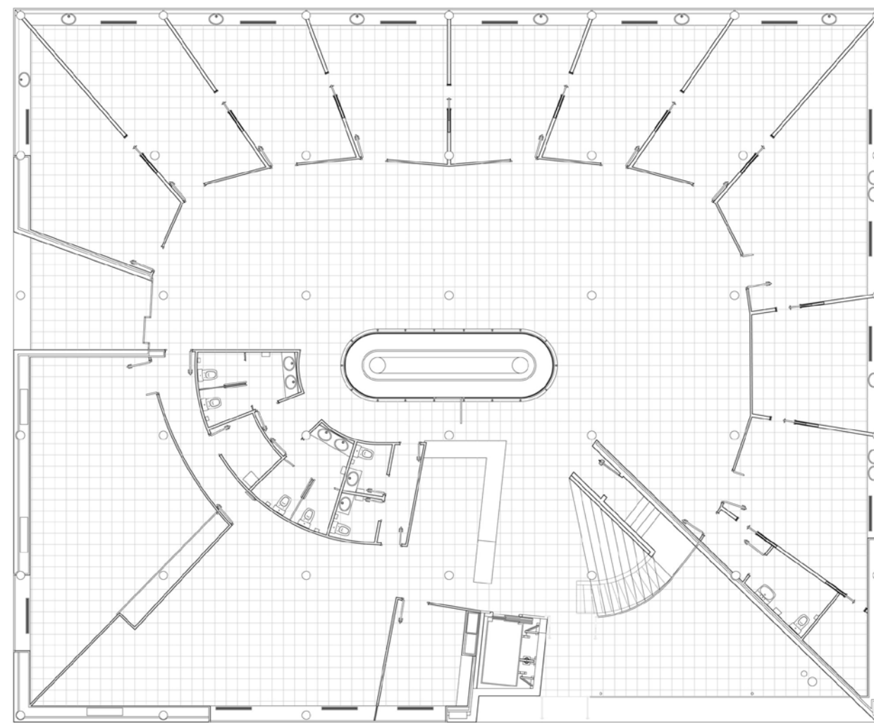
PLANTA BAJA/ GROUND FLOOR PLAN
